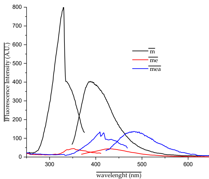
Figure S14. Fluorescence spectra of mea
