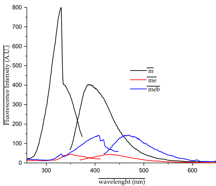
Figure S15. Fluorescence spectra of meb
