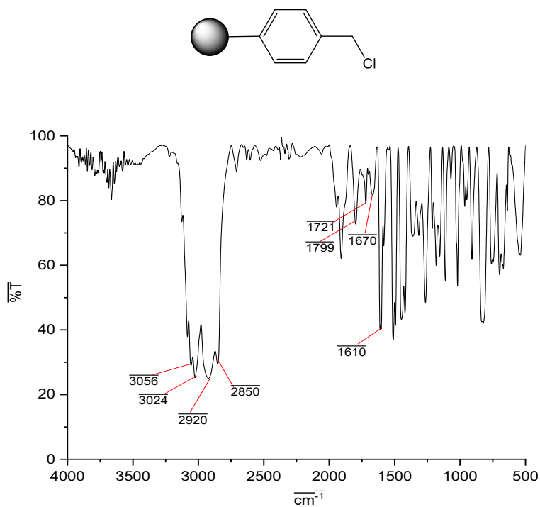
Figure S3. FT-IR spectrum of M
