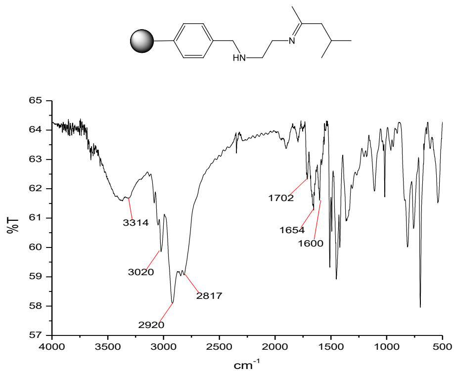
Figure S11. FT-IR spectrum of Meb
