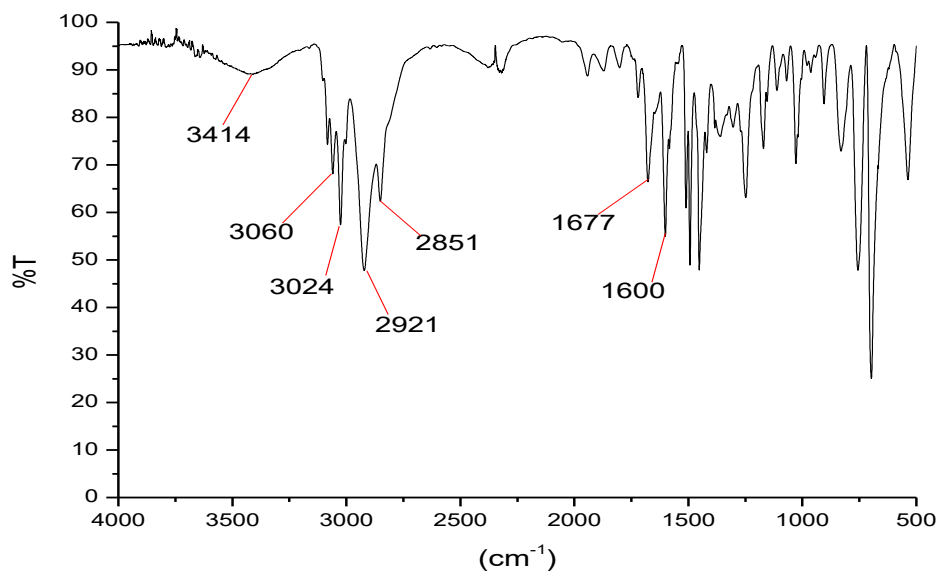
Figure S8. FT-IR spectrum of mec
