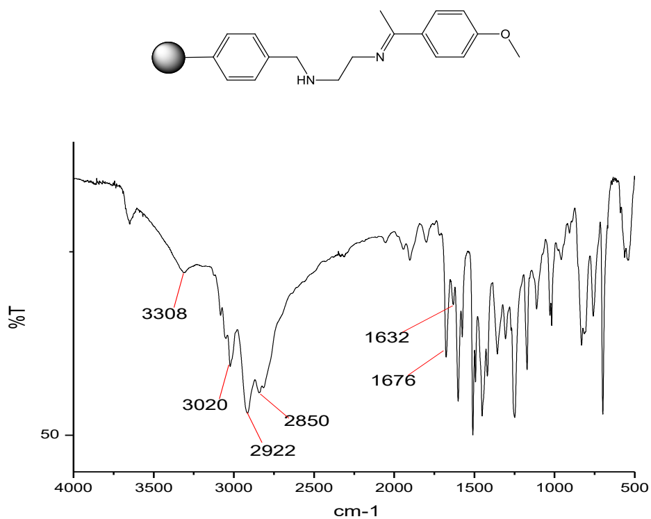
Figure S11. FT-IR spectrum of Meb
