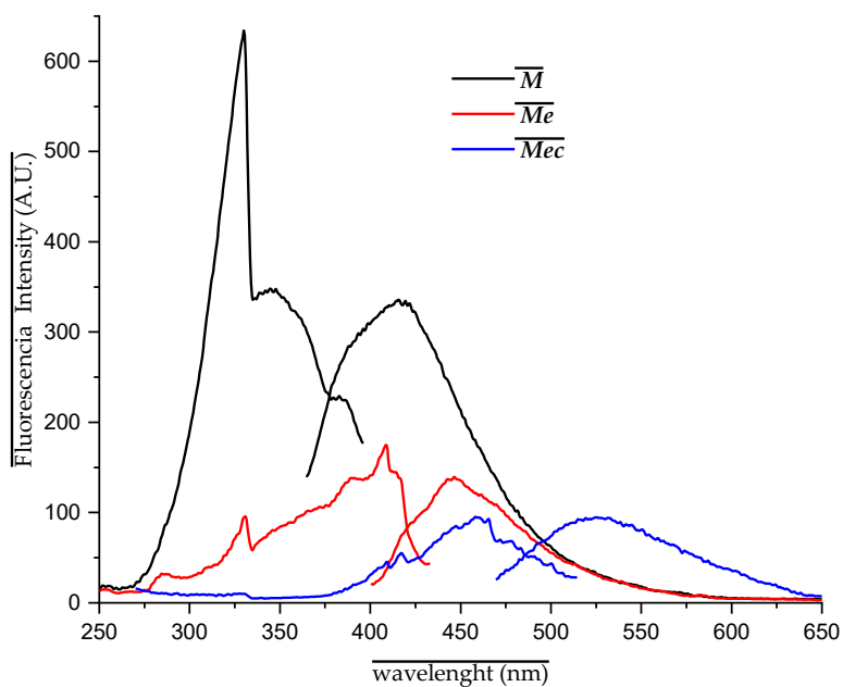
Figure S20. Fluorescence spectra of Mec
