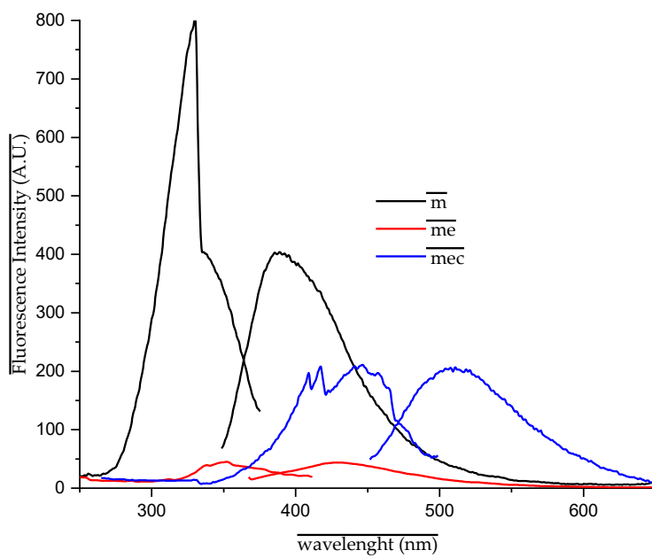
Figure S16. Fluorescence spectra of mec
