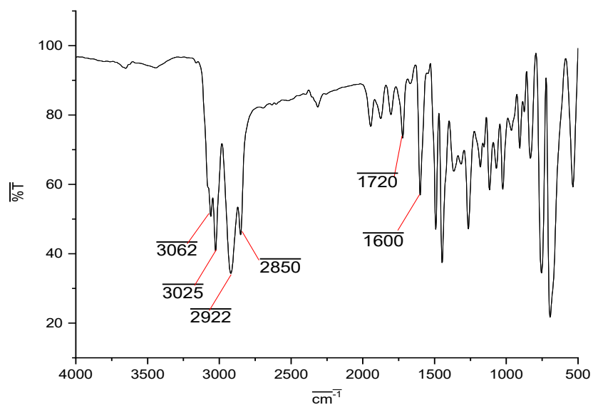
Figure S2. FT-IR spectrum of m
