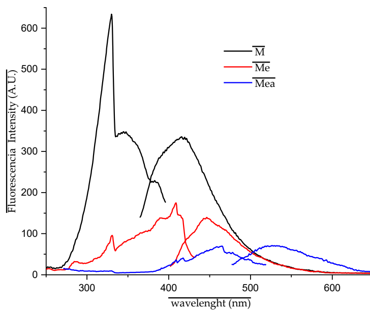
Figure S18. Fluorescence spectra of Mea
