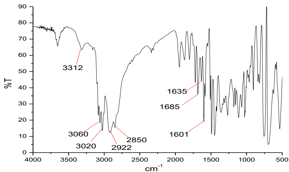
Figure S7. FT-IR spectrum of meb
