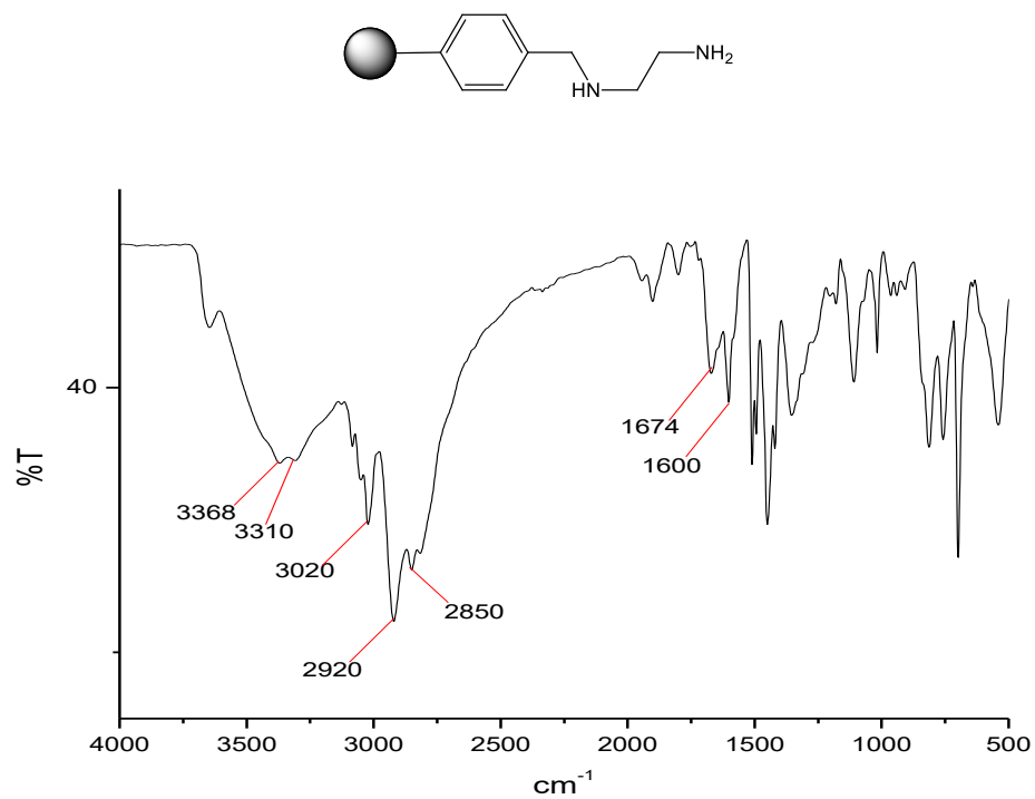
Figure S5. FT-IR spectrum of Me
