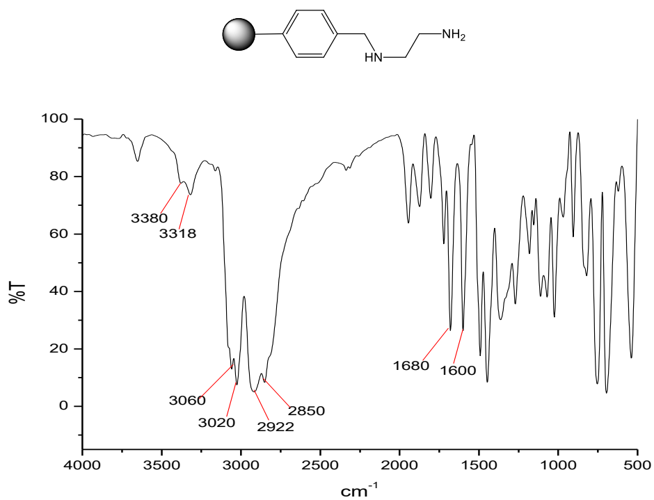
Figure S4. FT-IR spectrum of me
