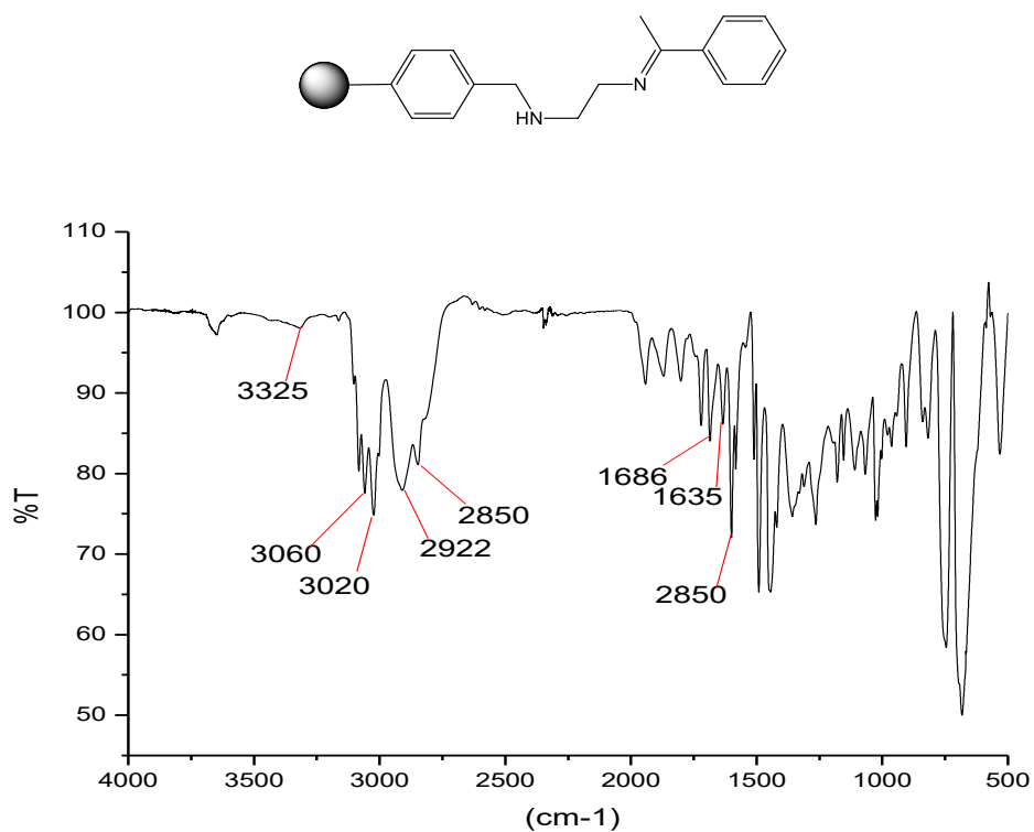
Figure S5. FT-IR spectrum of Me
